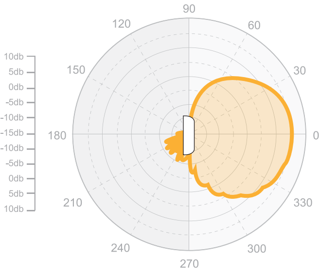
2.4 GHz, Horizontal
