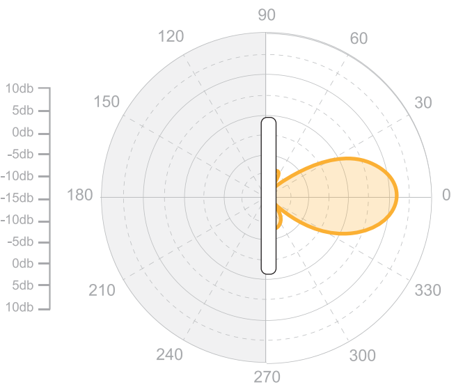
5 GHz, Vertical
