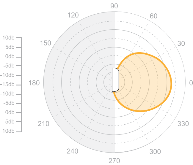
5 GHz, Horizontal
