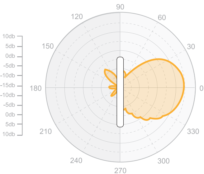
2.4 GHz, Vertical
