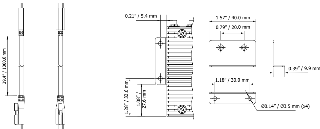
USB-C to USB-C Cable with Screw Locking (1 pc)
