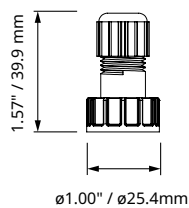
Waterproof Ethernet Connector (2 pcs, RJ45)
