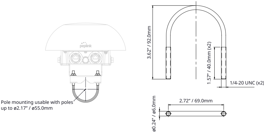
U-Bolt (2 pcs)
