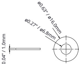
Washer (4 pcs)
