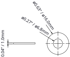
Washer (4 pcs, M6)
