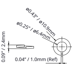
Spring Washer (4 pcs, M6)
