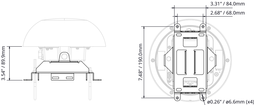
Mount Bracket (1 pc)
