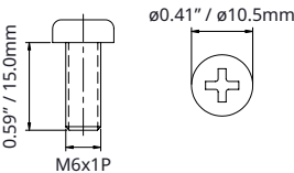
Screw (4 pcs, M6x15L)
