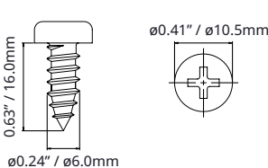
Screw (4 pcs, M6x16L)
